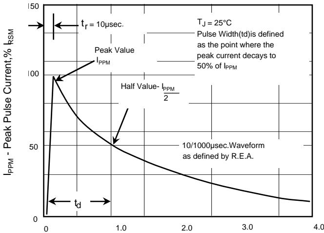
Fig. 3 - Pulse Waveform
